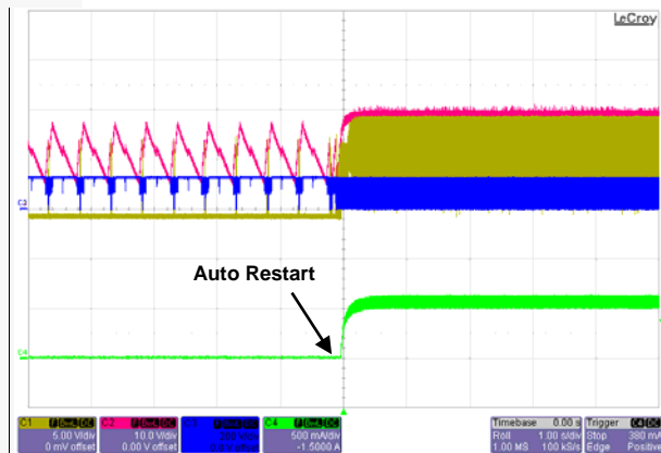
Figure 22. V_{IN} = 90 V_{AC} / 60 \text{ Hz} , [LED Restore]
