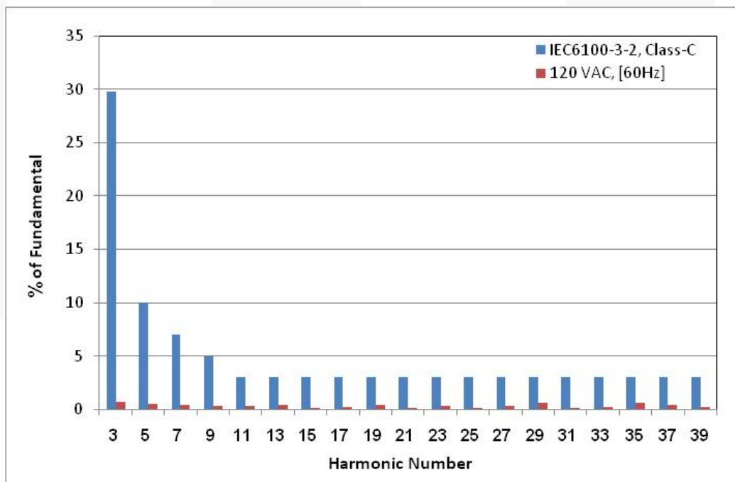
Figure 36. V_{IN} = 120 V_{AC} / 60 \text{ Hz}
