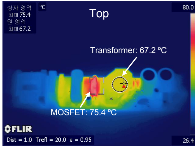
Figure 39. V_{IN} = 90 V_{AC} / 60 \text{ Hz}
