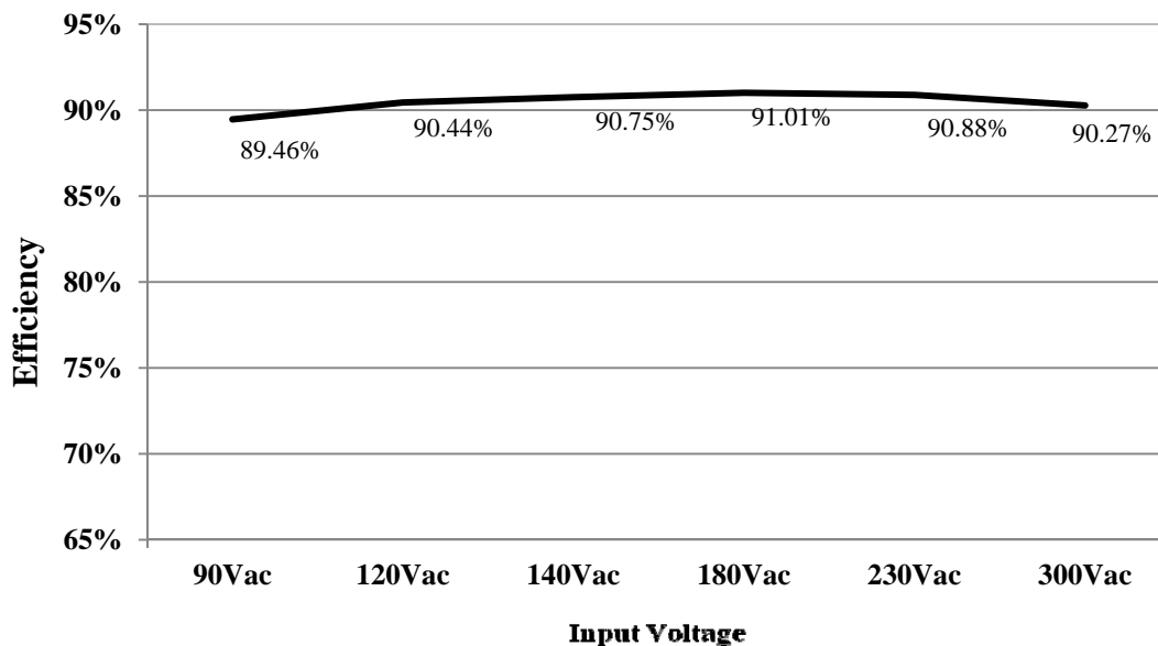
Figure 32. System Efficiency
