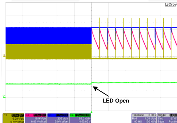
Figure 27. V_{IN} = 300 V_{AC} / 50 \text{ Hz} , [LED Open]
