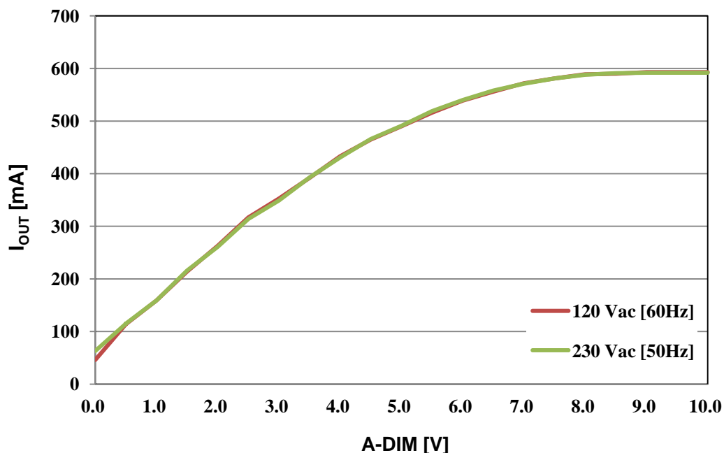
Figure 29. Analog Dimming
