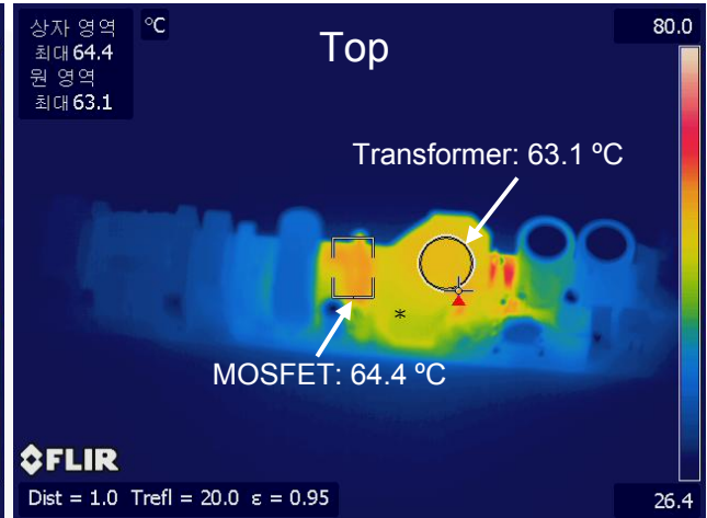
Figure 40. V_{IN} = 300 V_{AC} / 50 \text{ Hz}
