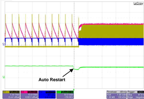
Figure 26. V_{IN} = 90 V_{AC} / 60 \text{ Hz} , [LED Restore]
