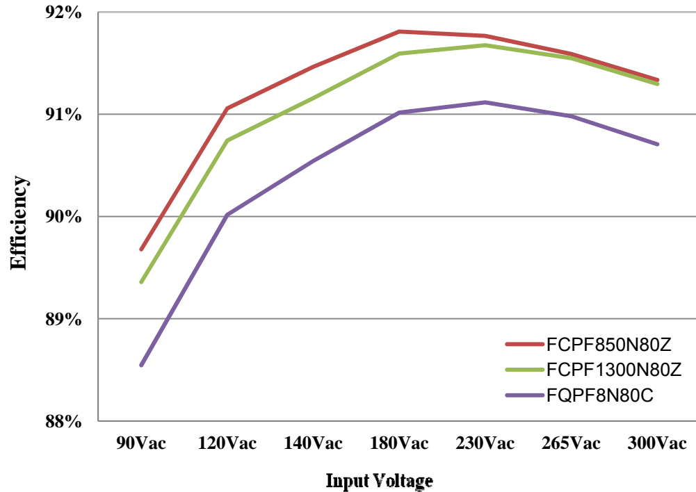
Figure 33. System Efficiency
