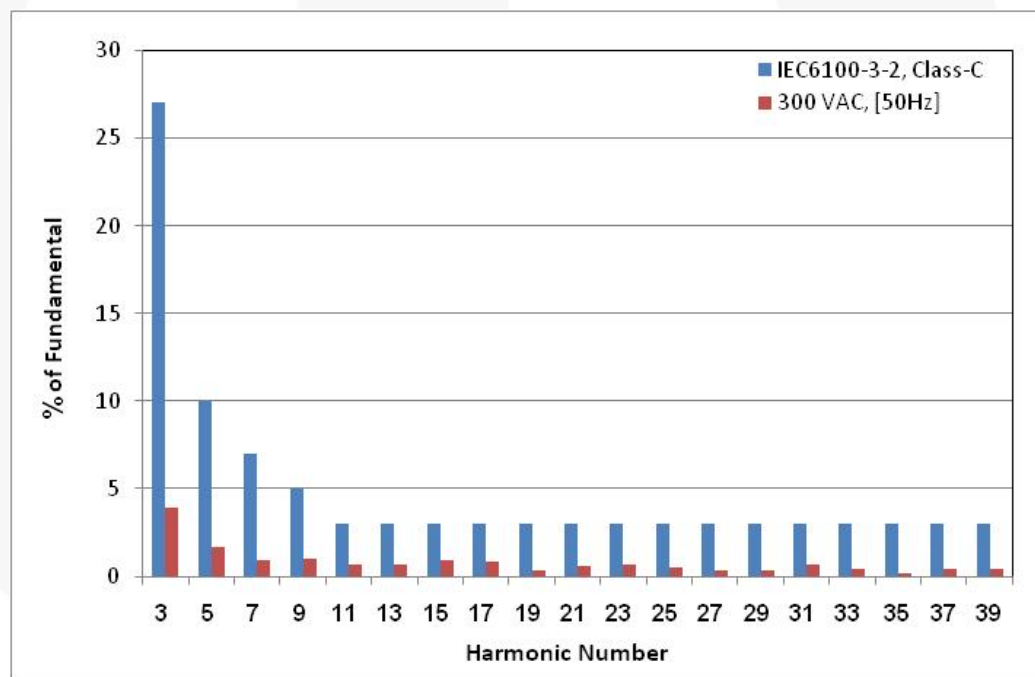
Figure 38. V_{IN} = 300 V_{AC} / 50 \text{ Hz}
