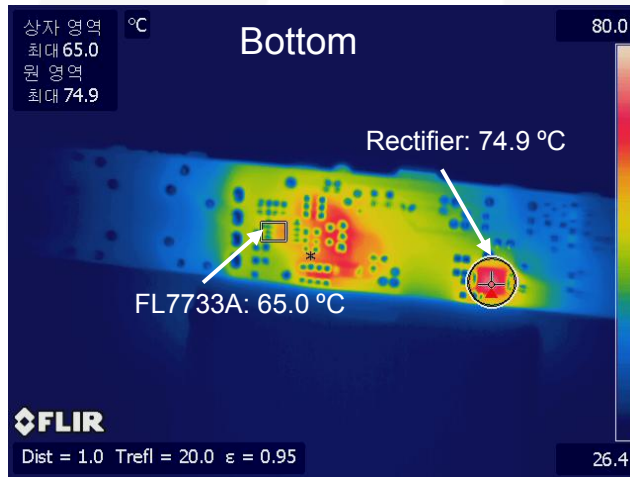
Figure 41. V_{IN} = 90 V_{AC} / 60 \text{ Hz}
