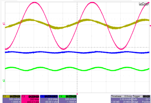
Figure 15. V_{IN} = 300 V_{AC} / 50 \text{ Hz}
