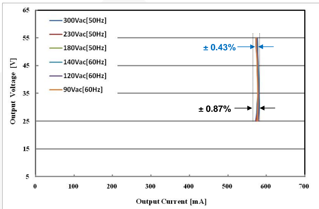
Figure 20. Constant-Current Regulation
