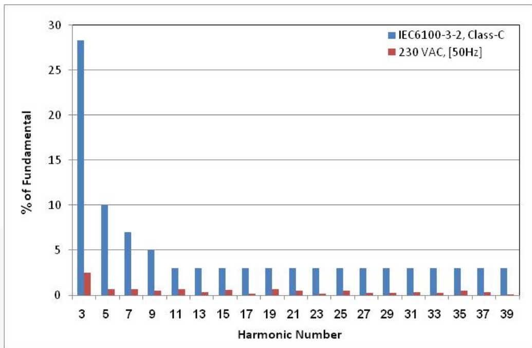
Figure 37. V_{IN} = 230 V_{AC} / 50 \text{ Hz}
