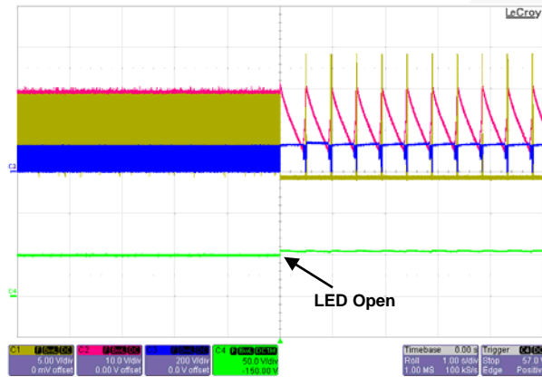
Figure 25. V_{IN} = 90 V_{AC} / 60 \text{ Hz} , [LED Open]
