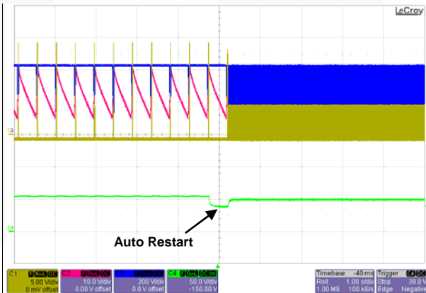
Figure 28. V_{IN} = 300 V_{AC} / 50 \text{ Hz} , [LED Restore]
