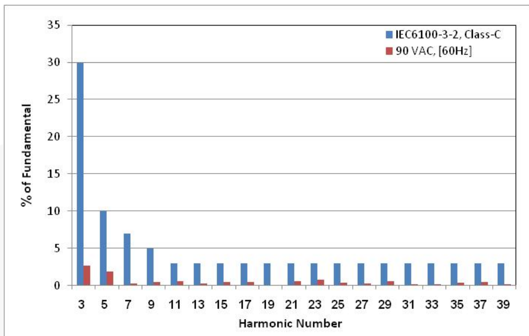
Figure 35. V_{IN} = 90 V_{AC} / 60 \text{ Hz}
